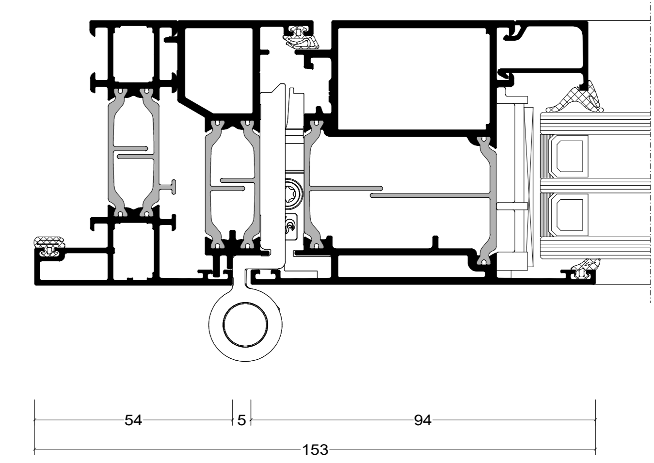
TRIPLE GLAS
